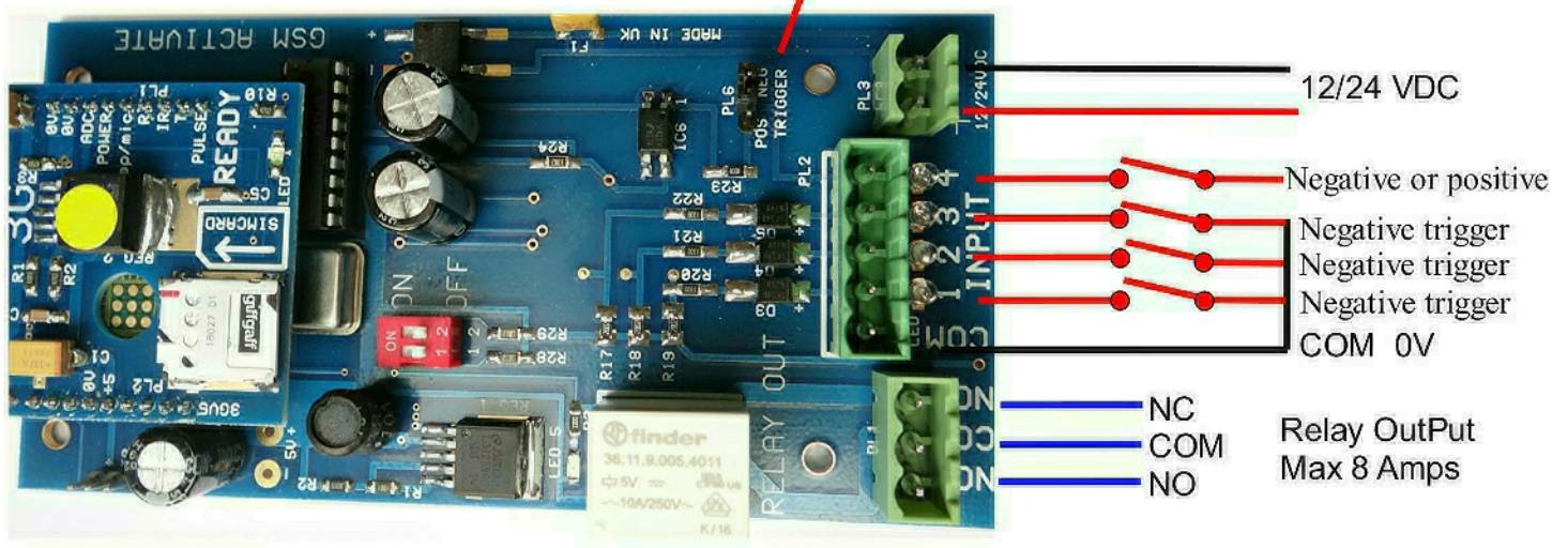
fig 1 TRIGGER LINK Input 4 only
